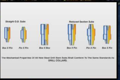
Straight OD Subs & Reduced Section Subs
